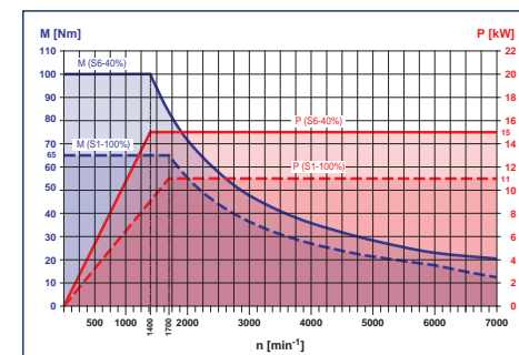
HYPERTURN 45-G3 main spindle / counter spindle
