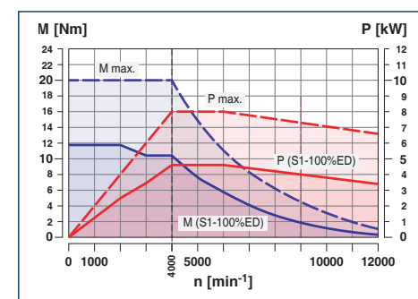
BMT45P tool turret with direct drive
