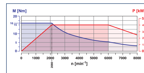
VDI25 tool turret with driven tools
