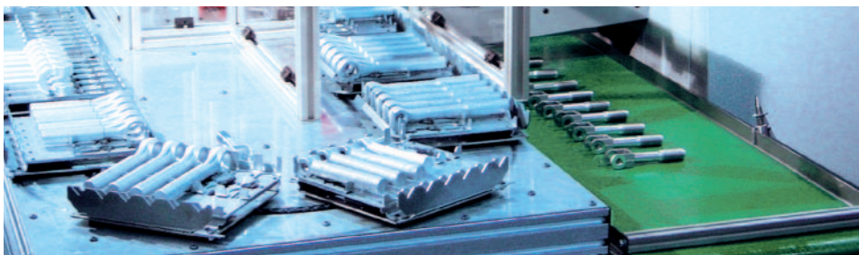
20-station pallet magazine with customer-specific pallets
