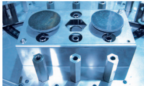
Multi-pallet attachment for a family of parts
