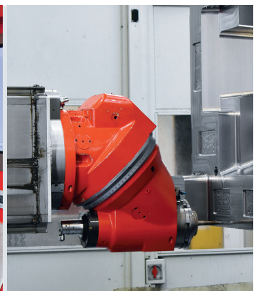
Continuously variable high-performance mechanical universal head for roughing and pre-finishing operations
