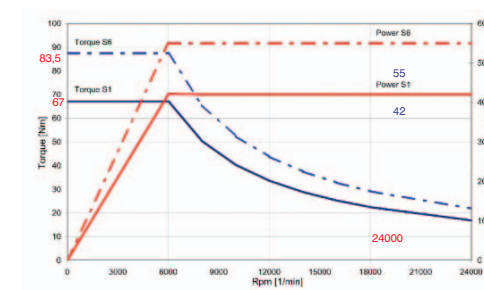
Universal milling head with torque motors and high speed spindle
