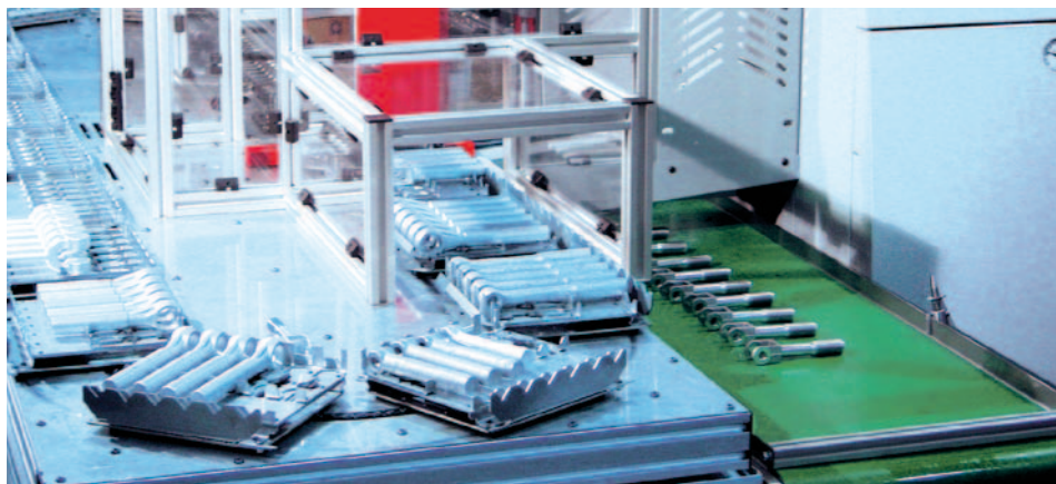
20-station pallet magazine with customer-specific pallets
