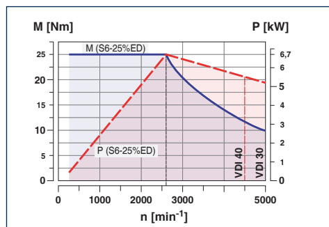
Milling drives in tool turret with VDI 30/40
