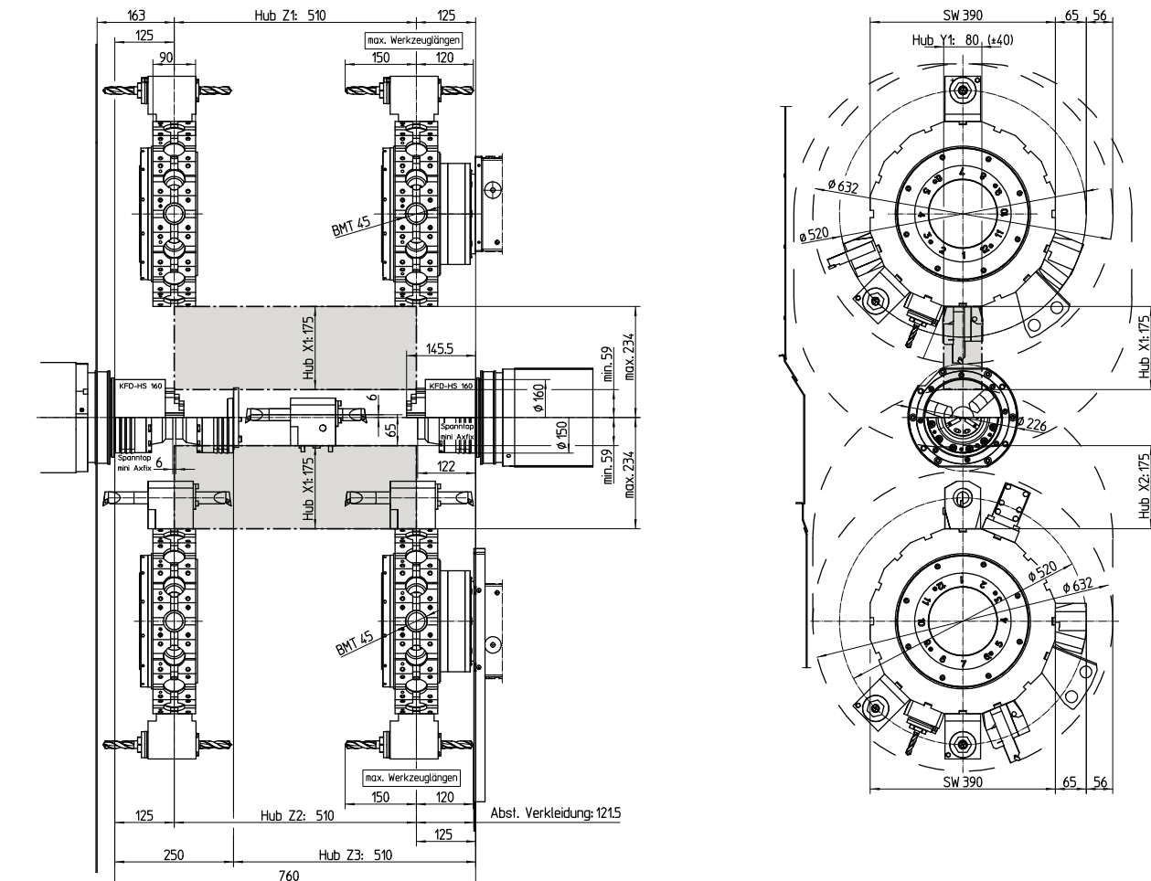
Work area HT45-G3 with 16-station BMT45P turret
